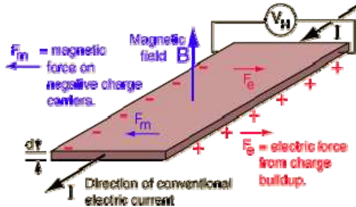
Fig.7 The Principle of Hall Effect
