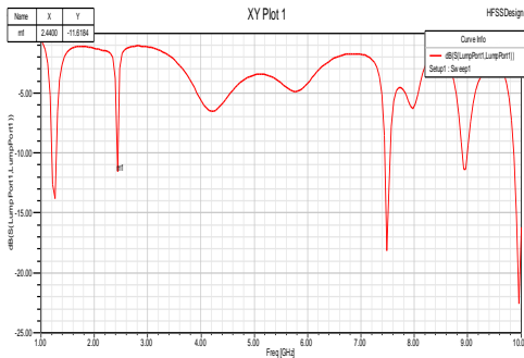
Fig.3. Frequency (GHz)
