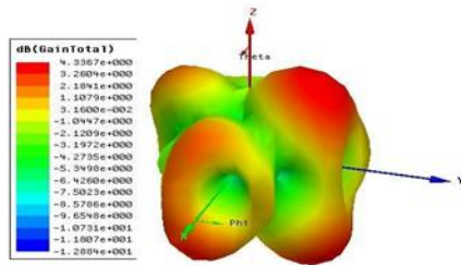
Fig.7.Total gain
