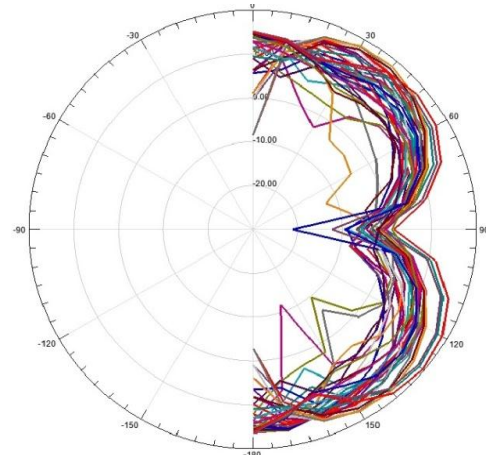
Fig.5. Radiation Pattern1 for E-Field
