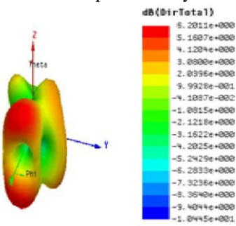
Fig.8. Total directivity
