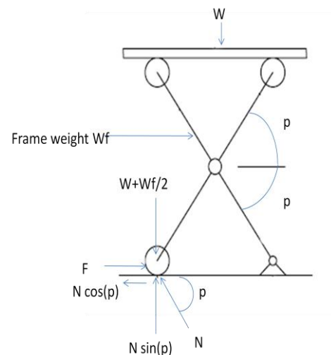
Fig.1. Reaction forces acting on Scissor lift
