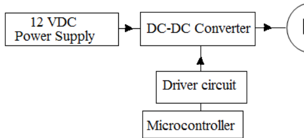
Figure 3: DC motor speed controller system with microcontroller.
