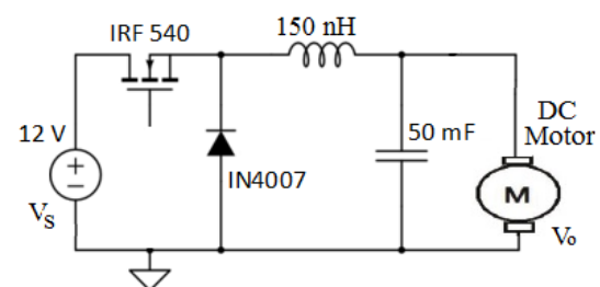
Figure 2: DC-DC Converter
